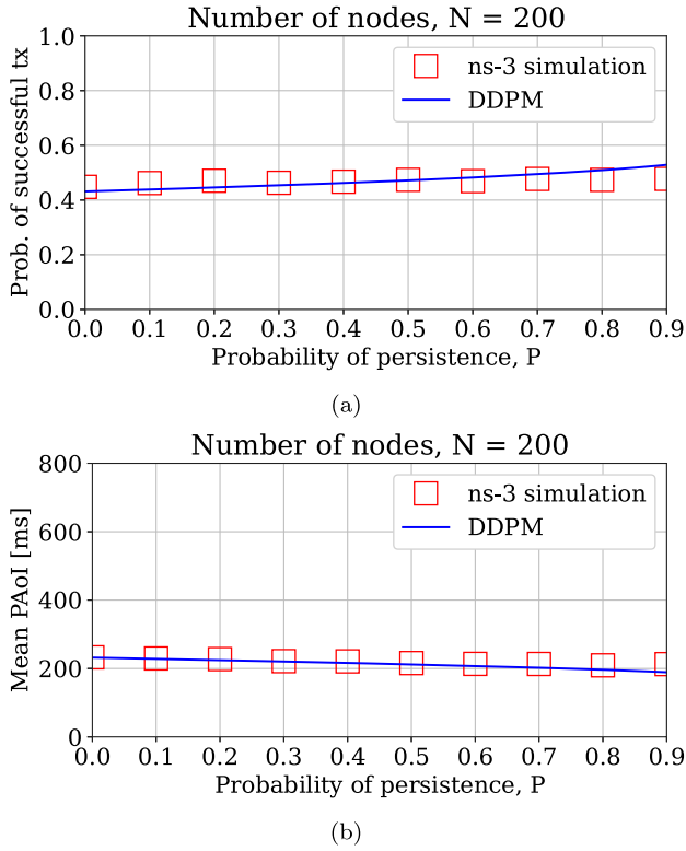
Fig. 20. Comparative analysis of (a) transmission success probability, and (b) mean PaoI between analytical model and ns-3 simulations with RC \in [5; 15] and for distances less than 800m.
