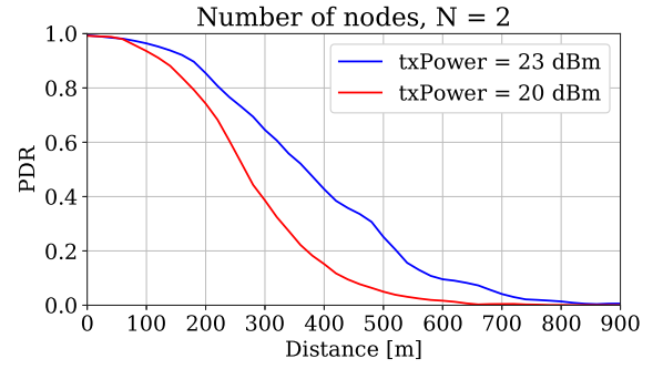
Fig. 11. PDR as a function of distance for one pair of nodes.
