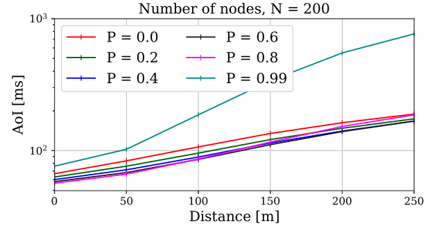
Fig. 15. AoI as a function of distance (log-scale).
