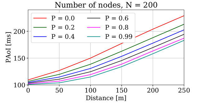
Fig. 14. PAoI as a function of distance.
